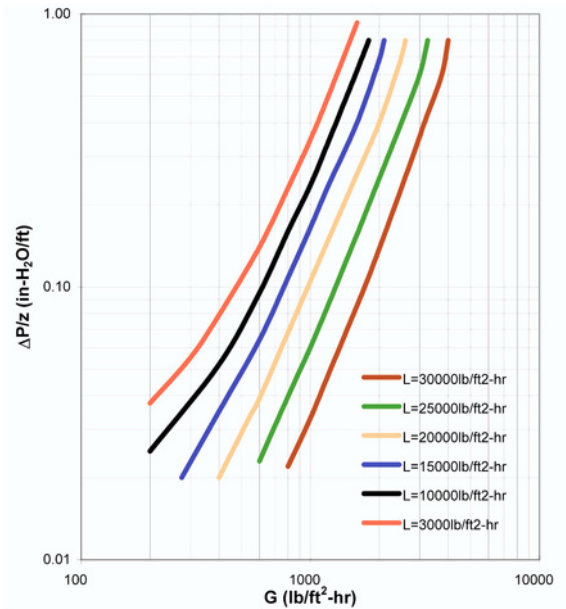
2" Globe-Pac™ Pressure Drop
