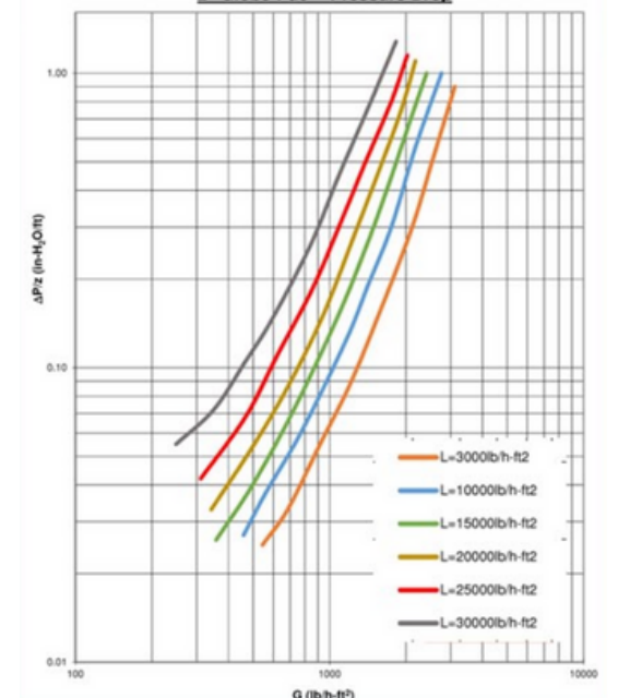
2" Globe-Pac™ Pressure Drop
